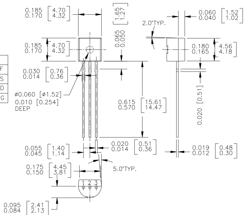
TO-92 (92,94,96)
